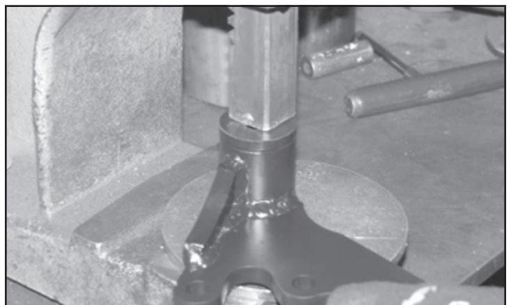
FIGURE 25 - STEP 24
