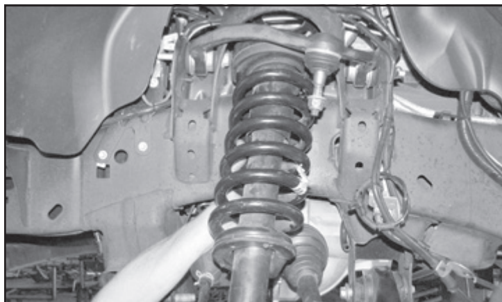
FIGURE 4 - STEP 10
