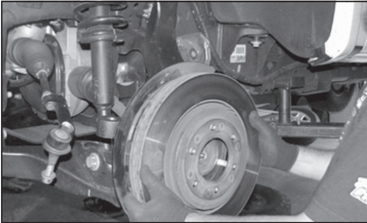
FIGURE 49 - STEP 50
